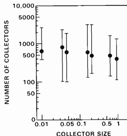
FIG. 4. Median ( N = 12 ) number versus size of collectors required to estimate monthly epiphyte biomass within \pm 10\% of the mean 90% of the time (bars represent range).
