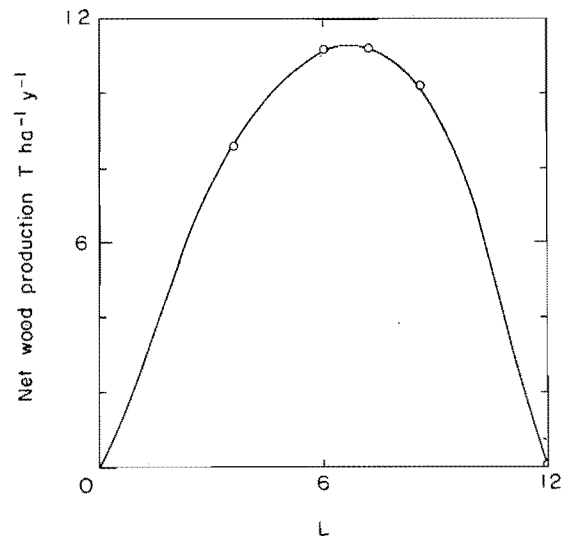
Fig. 9. When losses from mortality of more than 200 trees \text{ha}^{-1}\text{y}^{-1} were subtracted from gross wood production at the highest canopy density ( L ), net wood production approached zero. The general response is a parabolic curve rather than an asymptotic one, as illustrated in Fig. 8. Adapted from Waring et al. (1981).
