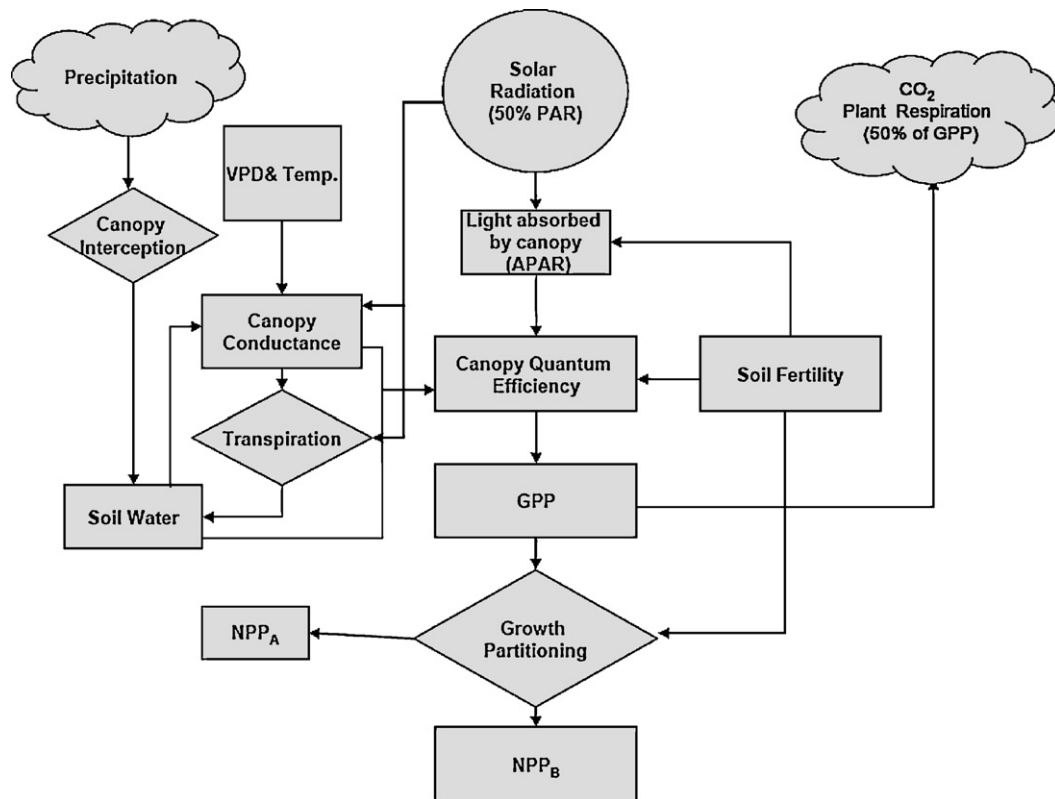
Fig. 1. Schematic diagram of the 3-PGS model. Gross ( GPP ) and net primary production ( NPP ) are ultimately functions of the amount of light absorbed by the canopy ( APAR ) and the canopy quantum efficiency ( \alpha ). Additional restrictions are imposed on photosynthesis through reduction in stomatal conductance ( g_s ; see text) if air temperatures, atmospheric humidity deficits ( VPD ) or the available soil water supply ( \theta ) are suboptimal. GPP is partitioned equally into NPP and autotrophic respiration. NPP is further partitioned into belowground ( NPP_B ) and above-ground ( NPP_A ) components depending on soil fertility and available water (modified from Coops et al., 1998).
