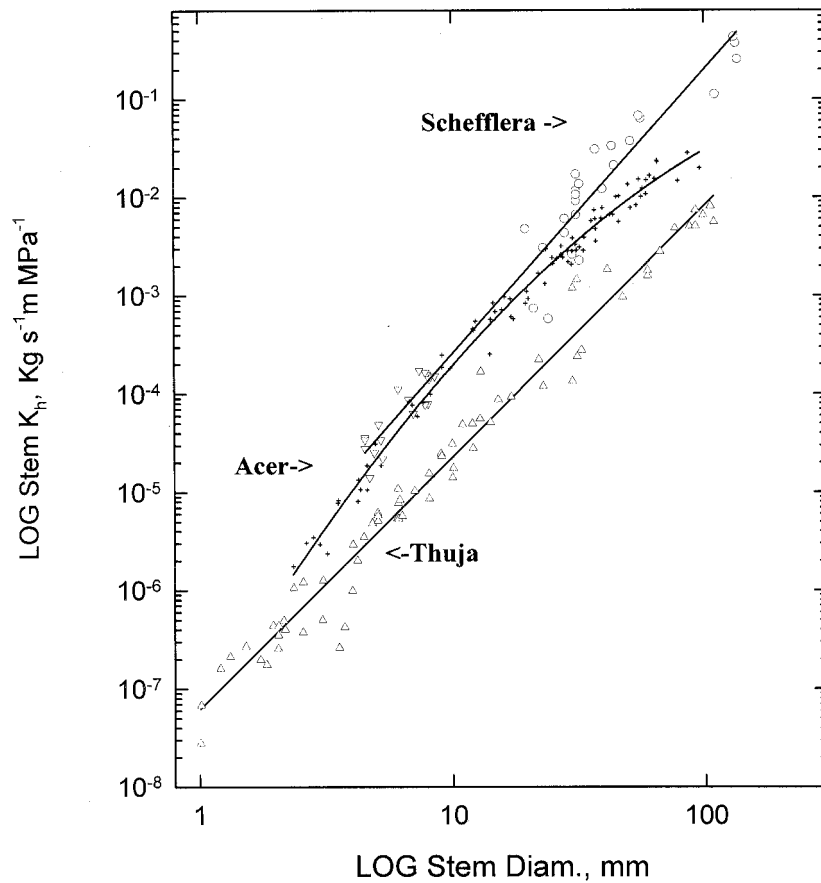
Fig. 4. Hydraulic conductivity of stems per unit pressure gradient, K_h , plotted versus diameter of the stem (excluding bark, x -axis). Species represented are Thuja occidentalis , Acer saccharum , and Schefflera morototoni . Both axes are logarithmic. Adapted from Tyree et al. (1991).
