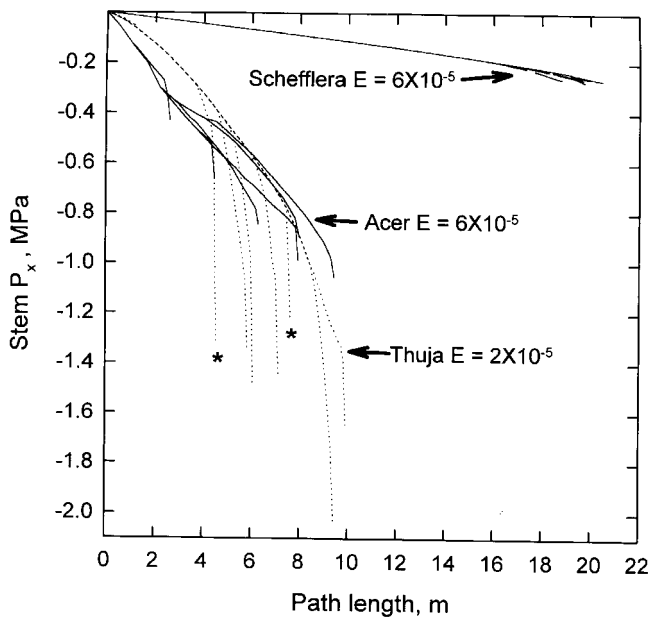
Fig. 6. Profiles of xylem pressure potential, P_x , versus distance water must travel from the base of the tree to a stem apex. All values include the gravitational potential gradient required to lift water up the tree. The curves were calculated from the hydraulic maps and the representative midday evaporative flux densities ( E ) indicated for each species in the graph. Adapted from Tyree et al. (1991).
