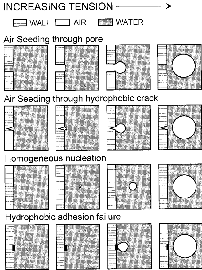
Fig. 8. Four possible mechanisms of cavitation induction. (1) Air-seeding through a pore occurs when the pressure difference across the meniscus is enough to allow the meniscus to overcome surface tension and pass through the pore. (2) Air-seeding through a hydrophobic crack occurs when a stable air bubble resides at the base of a hydrophobic crack in the wall of a xylem conduit. When the P_x becomes negative enough the bubble is sucked out of the crack. (3) Homogeneous nucleation involves the spontaneous generation of a void in a fluid. It is a random process requiring thermal motion of the water molecules. The hydrogen bonds at a specific locus are broken when all water molecules randomly move away from any locus at the same instant with sufficient energy to break all hydrogen bonds between water molecules. As the tension in the water increases the hydrogen bonds are stretched and weakened so the energy needed to break the bonds decreases making a homogeneous nucleation more likely. (4) Hydrophobic adhesion failure is similar to homogeneous nucleation except that hydrogen bonds are broken between water and a hydrophobic patch in the wall where the energy of binding between water and wall is reduced.
