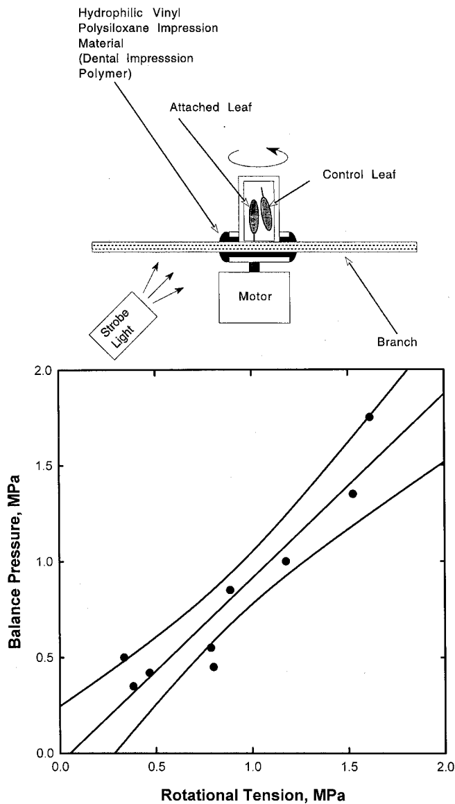
Fig. 3. The Holbrook experiment. (A) The experimental method. A stem segment was mounted on a centrifuge motor. Centrifugation of the segment induced a P_x as given in Equation 5. The strobe light was used to measure angular velocity. (B) Results show that the rotational tension was transmitted to the attached leaf; the x -axis is the calculated rotation tension= P_x in Equation 5 and the y -axis is the balance pressure of the attached leaf at the end of the experiment.
