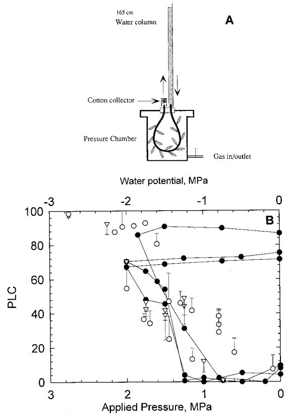
Fig. 9. The first experimental test of the air-seeding hypothesis. (A) The experimental apparatus. A willow branch is bent around in a large pressure bomb so that both cut surfaces are outside the bomb. Water continually passes through the stem segment under positive pressure from a water column to a cotton collector. Flow rate is estimated by measuring the weight change of the cotton collector over known time intervals. (B) The results are shown as a vulnerability curve where the y-axis is the per cent loss of hydraulic conductivity (PLC) and the x-axis is the negative P_x or the air pressure in the bomb needed to cause the plotted PLC. Open symbols are for PLC induced by negative P_x and closed symbols are induced by positive pressure applied in the pressure bomb. See text for more details.
