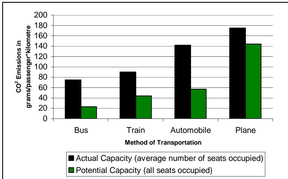
Figure 1: Carbon dioxide emissions of different modes of transportation (data adapted from Environment Canada http://www.ec.gc.ca/soer-ree/English/Indicators/Issues/Transpo/Tech_Sup/ptsup2_e.cfm )
