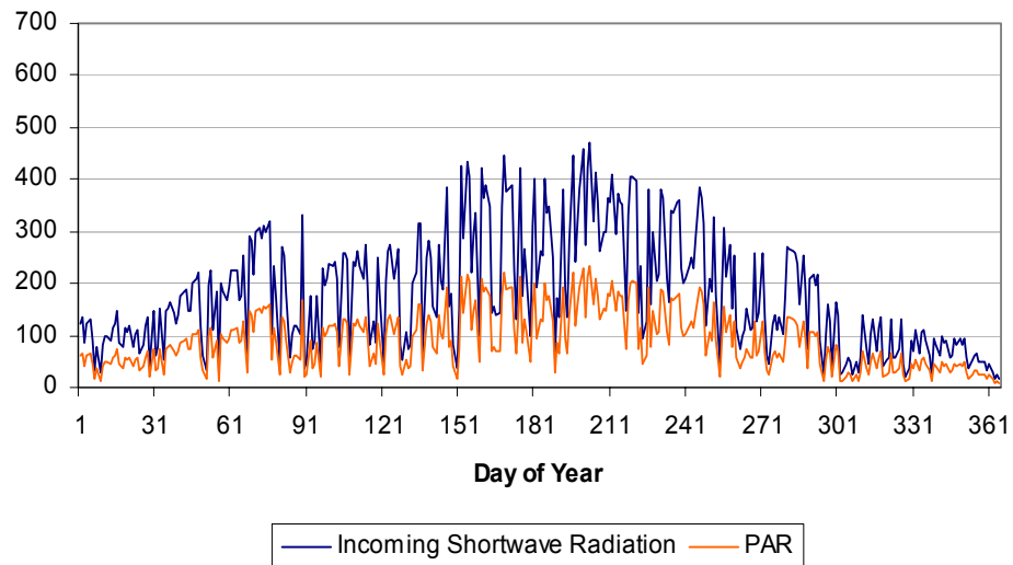
NOBS 2000 Radiation (W/m2)
