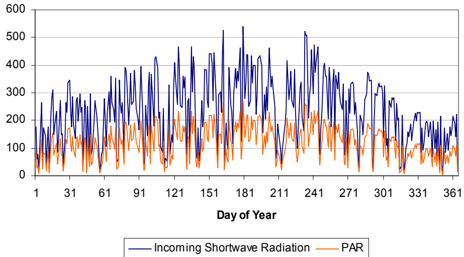
HARV 2000 Radiation (W/m2)
