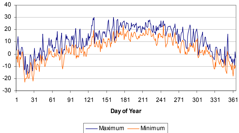
HARV 2000 Temperature (degC)
