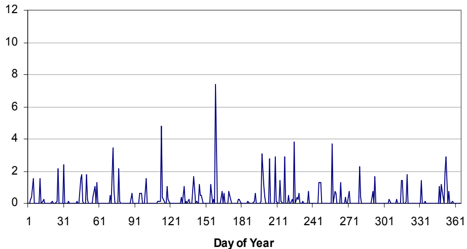
HARV 2000 Precipitation (cm)
