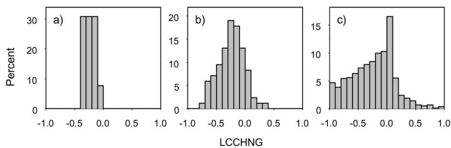
Figure 3. Probability distribution of LCCHNG summarized by (a) Subbasin; (b) Watershed; (c) Subwatershed.
